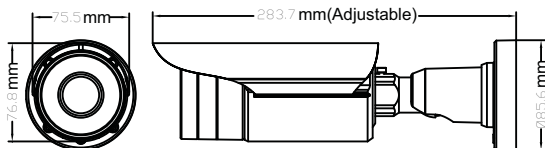
Photo 3-4 Outdoor IR Bullet Camera
